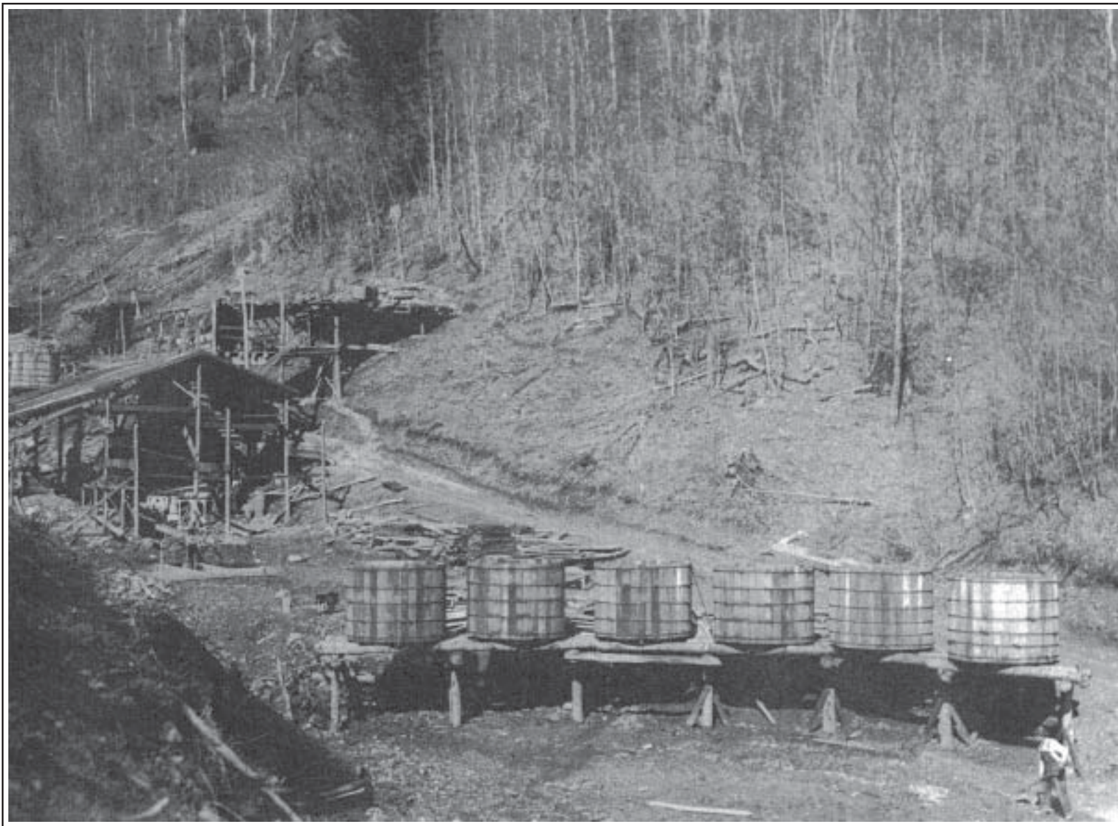
Figure 4.20. Structures and settling tanks at Adams Mine.
